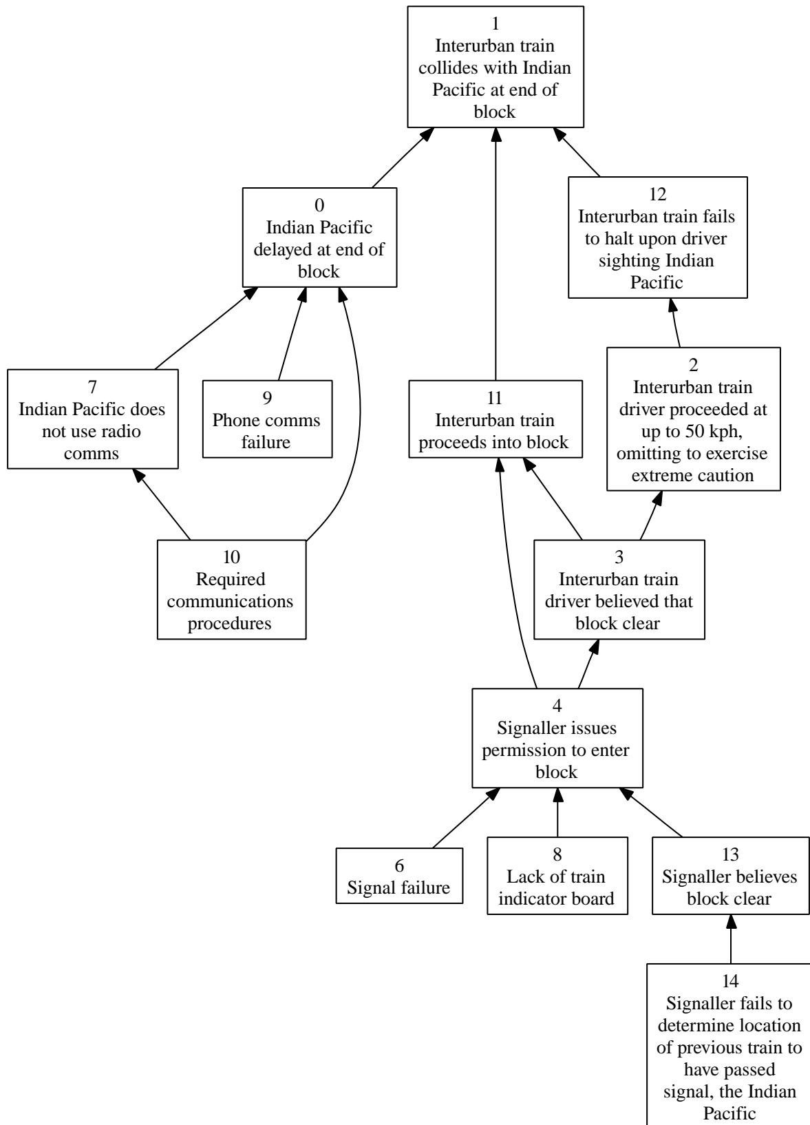
Fig. 2. The Glenbrook WB-Graph with Narrow Stopping Rule (WBG-NSR)
